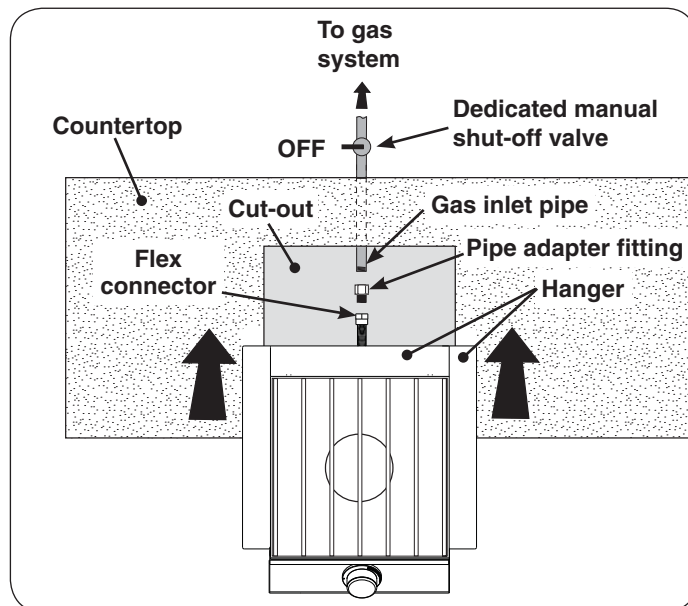
Fig. 12-3 Gas connection diagram
